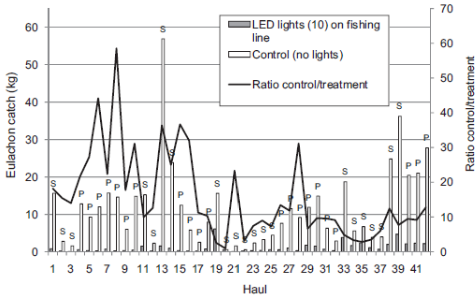
Figure 2-7. Haul-by-haul comparison of the catch of eulachon (kg) in the two nets of a double-rigged shrimp trawl vessel with one side incorporating 10 LED lights on the fishing line and the other acting as a control. The ratio of control/treatment catch is also shown (solid line). Label “P” or “S” denotes the side of trawl gear (port or starboard) used as the control net (Hannah et al. 2015).
