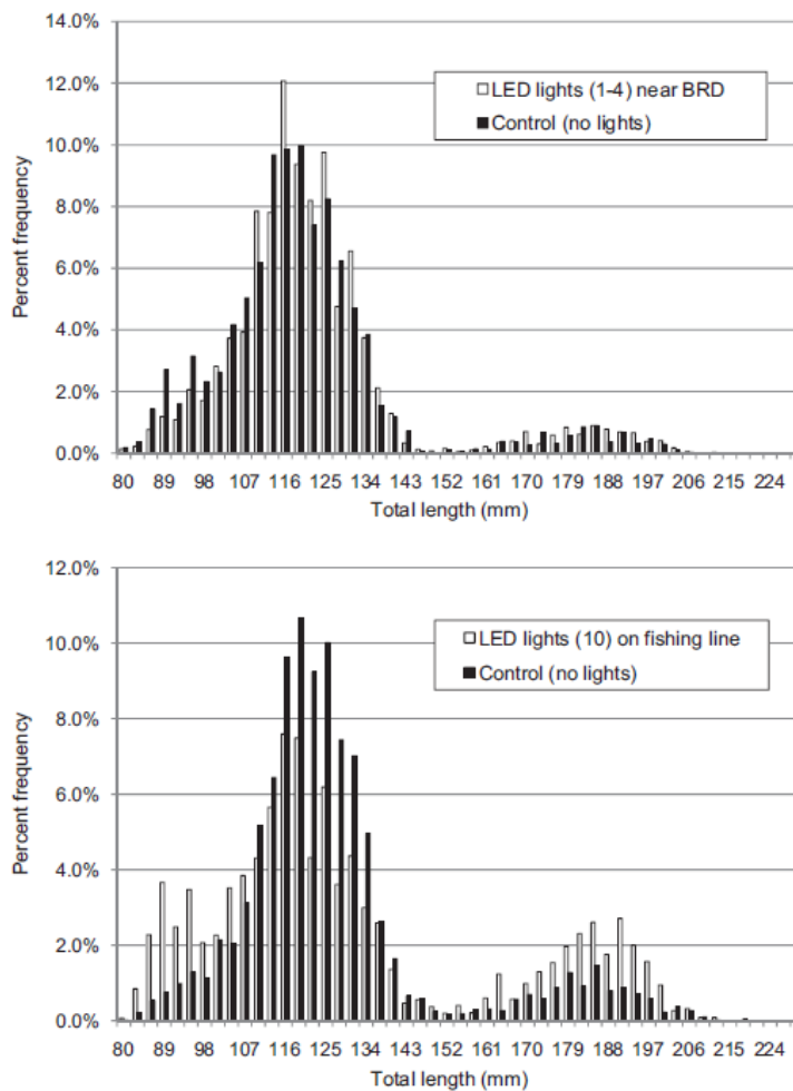
Figure 2-6. Percent length frequency of eulachon (total length, mm) captured in ocean shrimp trawl nets with and without 1–4 LED lights attached in the vicinity of the bycatch reduction device (upper panel) and with and without 10 LED lights attached to the trawl fishing line (lower panel). (Hannah et al. 2015).
