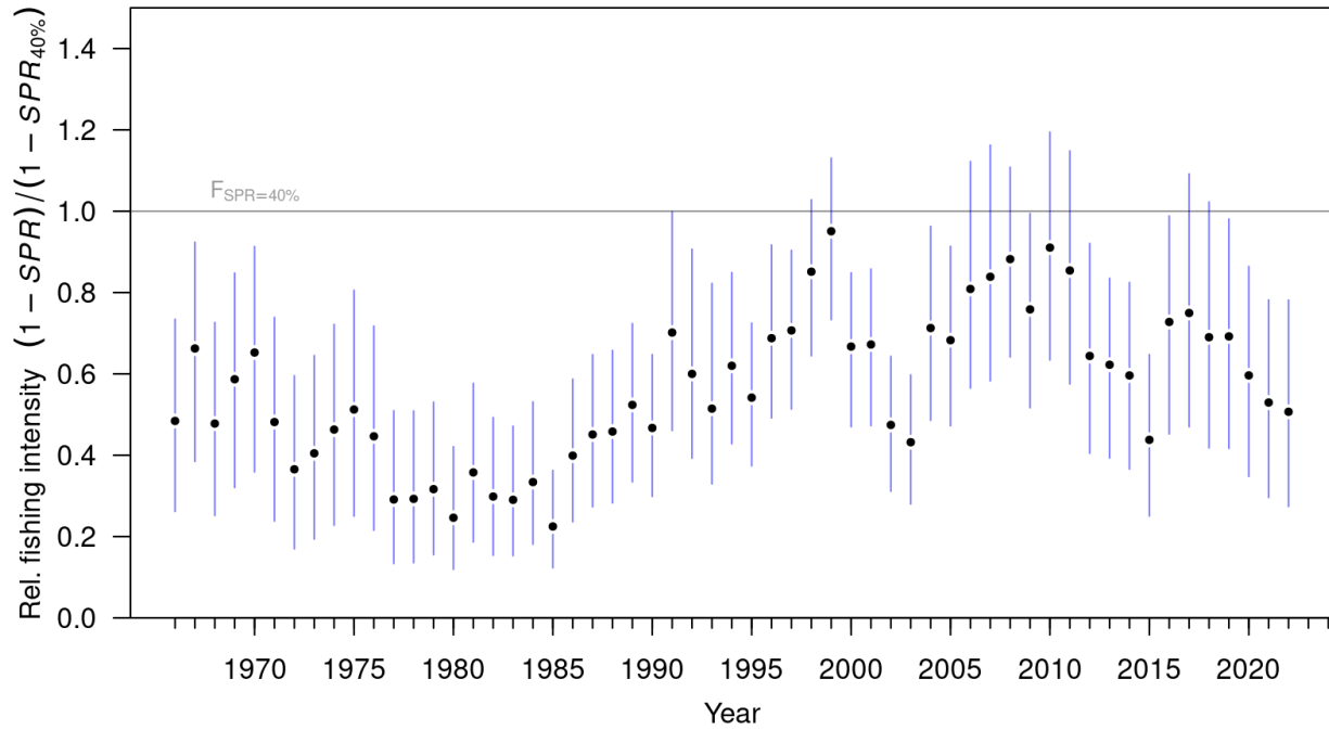
Figure 33. Trend in median fishing intensity (relative to the SPR management target) through 2022 with 95% posterior credibility intervals. The management target defined in the Agreement is shown as a horizontal line at 1.0.
