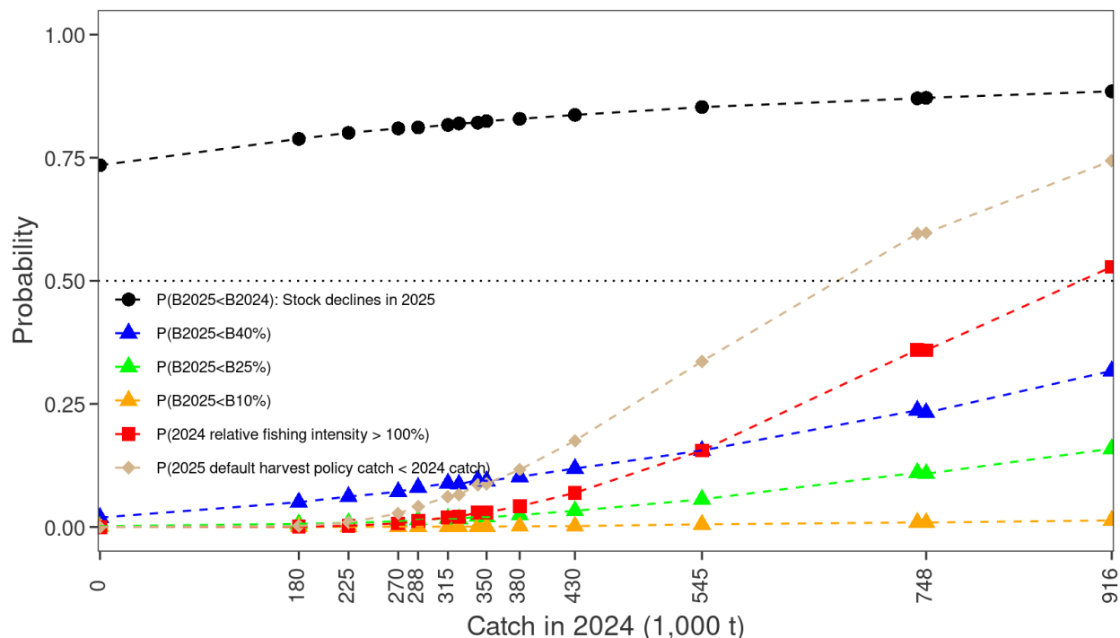
Figure i. Graphical representation of the probabilities related to spawning biomass, relative fishing intensity, and the 2025 default harvest policy catch for alternative 2024 catch options (including associated 2023 catch; catch options explained in Table g) as listed in Table j. The symbols indicate points that were computed directly from model output and lines interpolate between the points.
