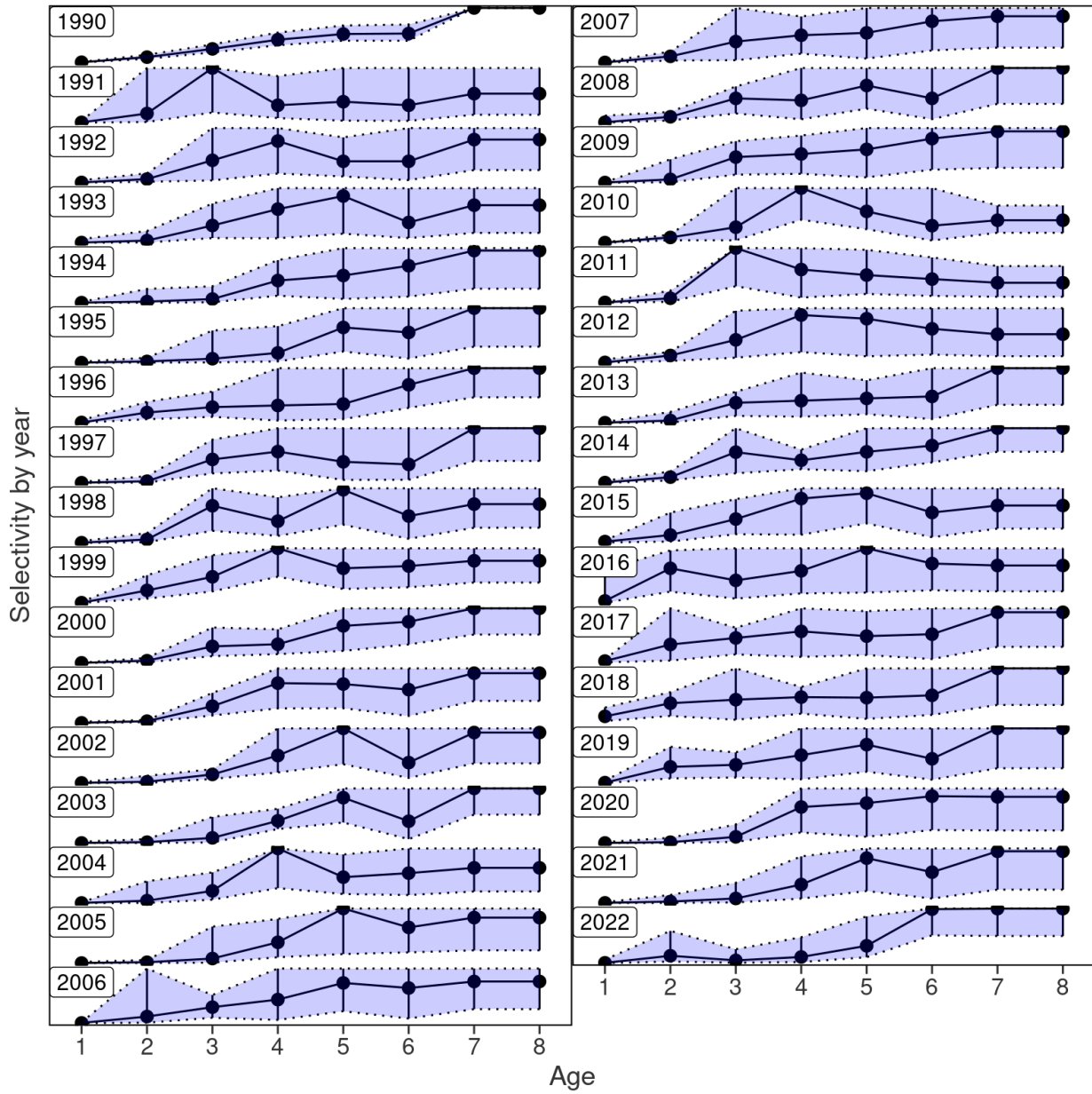
Figure B.5. As for Figure B.4 but with maximum age of estimated selectivity set to 7.
