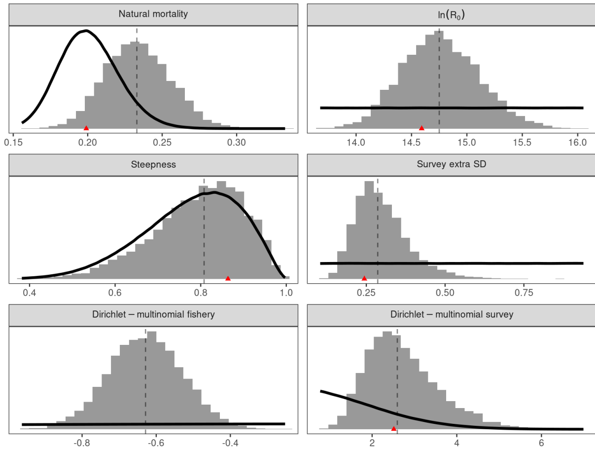
Figure 22. As for Figure 21 but the x axis of each panel is truncated to the range of the posterior distribution, and thus, there is the potential for the full range of the prior and the initial value to be missing from individual panels.
