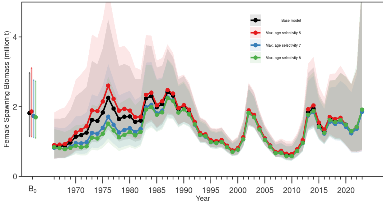
Figure B.3. Estimates of female spawning biomass for the base model and alternative sensitivity runs representing changing the maximum age of estimated fishery selectivity from the base model value of 6 to 5, 7, and 8.
