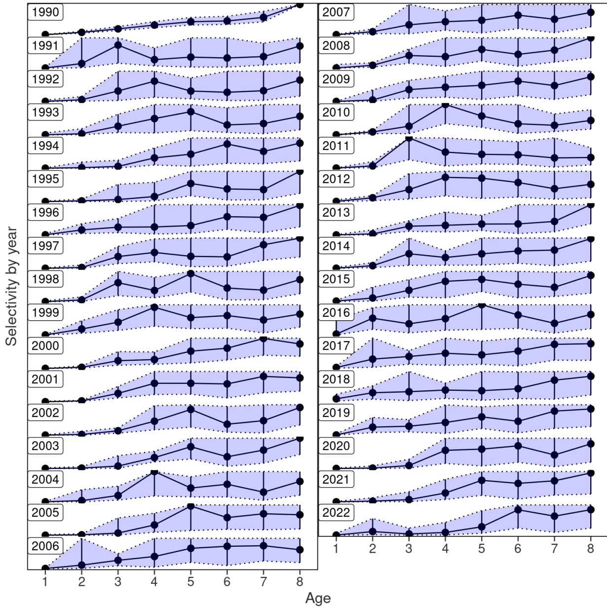
Figure B.6. As for Figure B.4 but with maximum age of estimated selectivity set to 8.
