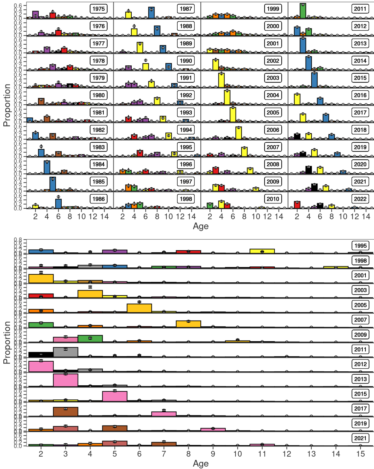
Figure 19. Base model fits to the observed fishery (top) and acoustic survey (bottom) age-composition data. Colored bars show observed proportions with colors following each cohort across years. Points with intervals indicate median expected proportions and 95% credibility intervals from the MCMC calculations.
