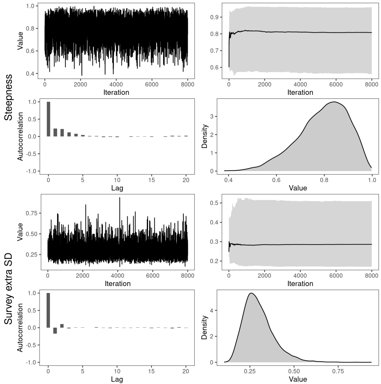
Figure A.2. Summary of Markov chain Monte Carlo diagnostics for steepness (upper panels) and the additional standard deviation (SD) in the biomass index (lower panels) in the base model. Sub-panel descriptions as in Figure A.1.
