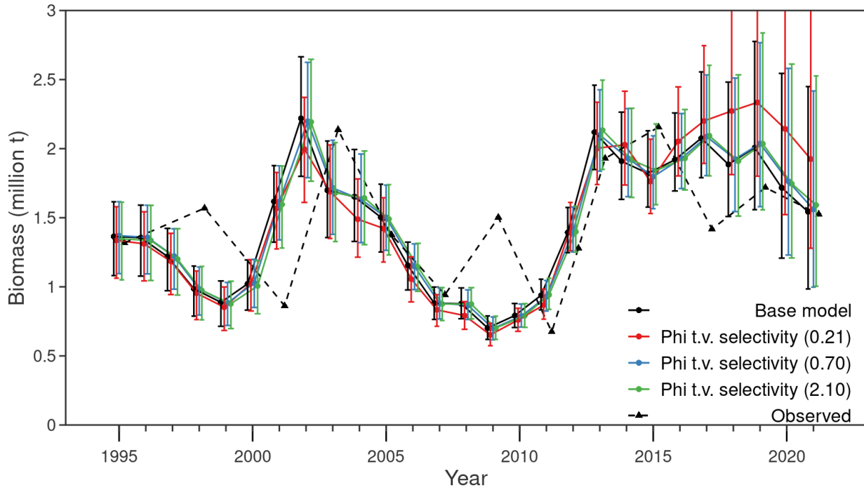
Figure 52. MCMC estimates of the fit to the survey index of age-2+ biomass for the base model and alternative sensitivity runs representing different standard deviations ( \Phi ) associated with time-varying selectivity. See Figure 48 for sensitivity descriptions.
