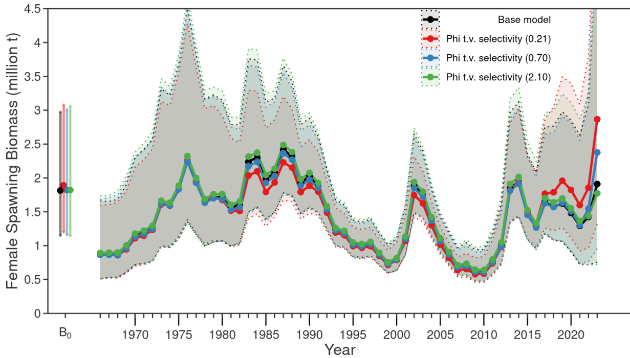
Figure 48. MCMC estimates of spawning biomass for the base model and alternative sensitivity runs representing different standard deviations ( \Phi ) associated with time-varying selectivity. Standard deviations examined are below (0.21 and 0.70) and above (2.10) the base model value of 1.4.
