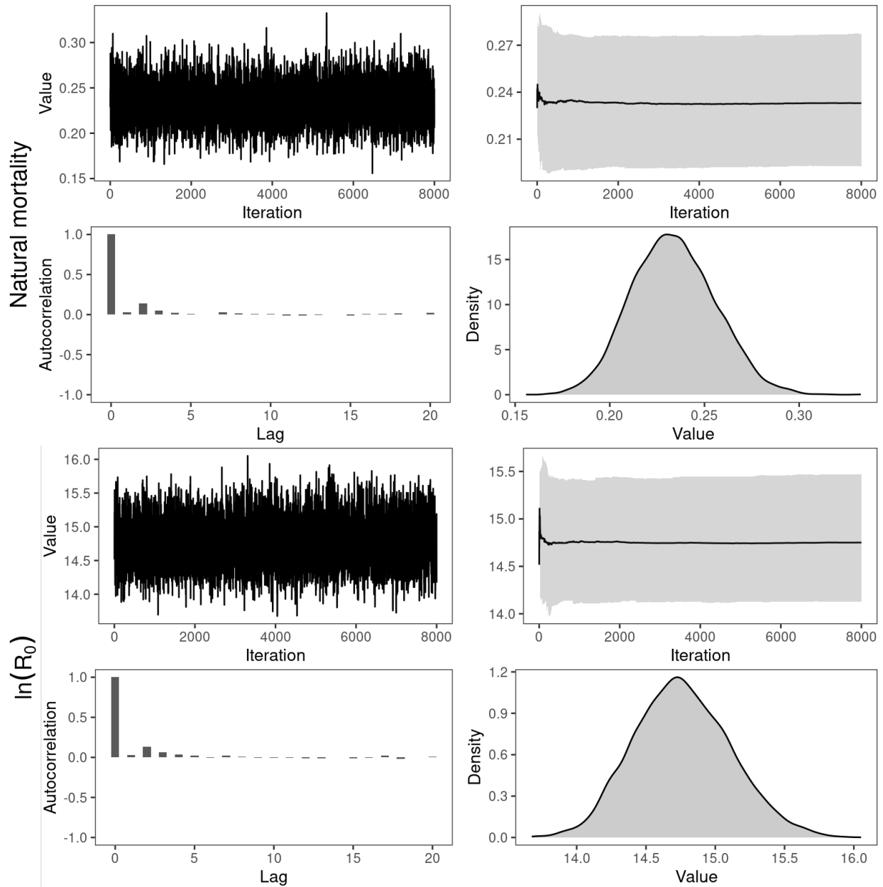
Figure A.1. Summary of Markov chain Monte Carlo diagnostics for natural mortality (upper panels) and the natural log of mean unfished equilibrium recruitment ( \ln(R_0) ; lower panels) in the base model. Top sub-panels show the trace of the sampled values across iterations (absolute values, top left; cumulative running median with 2.5th and 97.5th percentiles, top right). The lower left sub-panel indicate the autocorrelation present in the chain at different lag times (i.e., distance between samples in the chain), and the lower right sub-panel shows the distribution of the values in the chain (i.e., the marginal density from a smoothed histogram of values in the trace plot).
