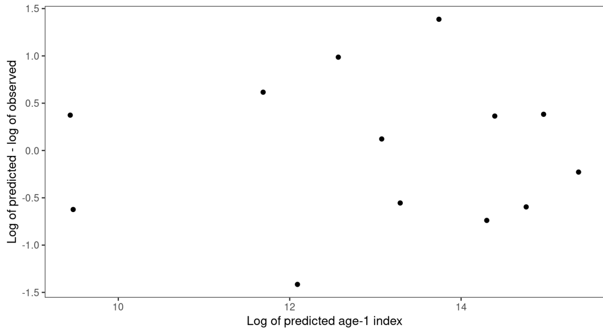
Figure B.2. As for Figure B.1 but on logarithmic axes.
