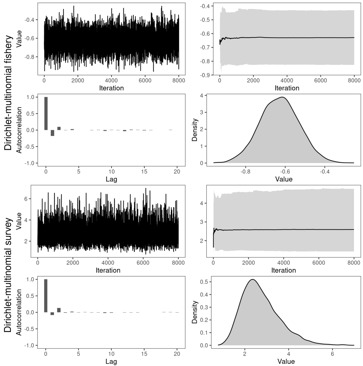
Figure A.3. Summary of Markov chain Monte Carlo diagnostics for the Dirichlet-multinomial age-composition parameters for the fishery ( \theta_{fish} , upper panels) and the survey ( \theta_{surv} , lower panels) in the base model. Sub-panel descriptions as in Figure A.1.
