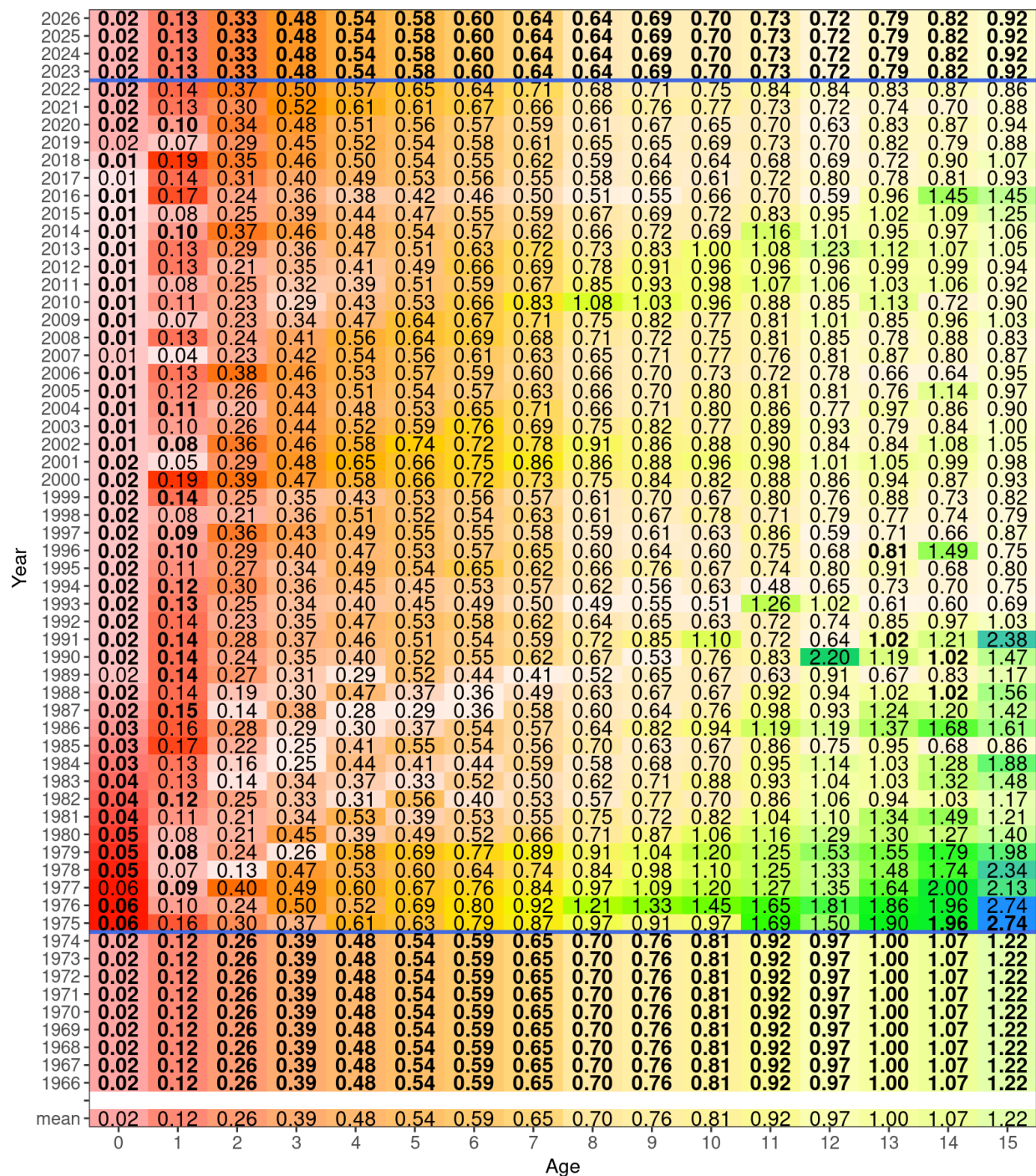
Figure 13. Empirical weight-at-age (kg) values used for the base model. Colors correspond to the values, with red being the lightest fish (across all years and ages) and blue being the heaviest fish. For each age, the most transparent cells indicate the lightest fish of that age. Data are only available from 1975–2022. Values based on assumptions for the pre-1975 and forecast years are shown outside the blue lines. Bold values between 1975–2022 represent unavailable data such that weights were interpolated or extrapolated from adjacent ages or years. The bottom row (mean) is the sample-weighted mean weight-at-age over all years of data.
