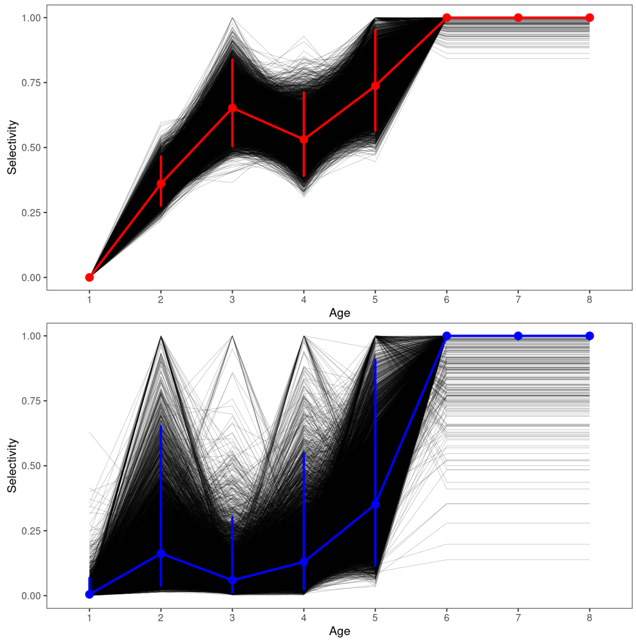
Figure 25. Estimated selectivities for the acoustic survey age-2+ biomass index (top, with selectivity of zero for age-1 fish) and fishery (bottom – shown for 2022 only, age-1 and older) from the posterior distribution for the base model.
