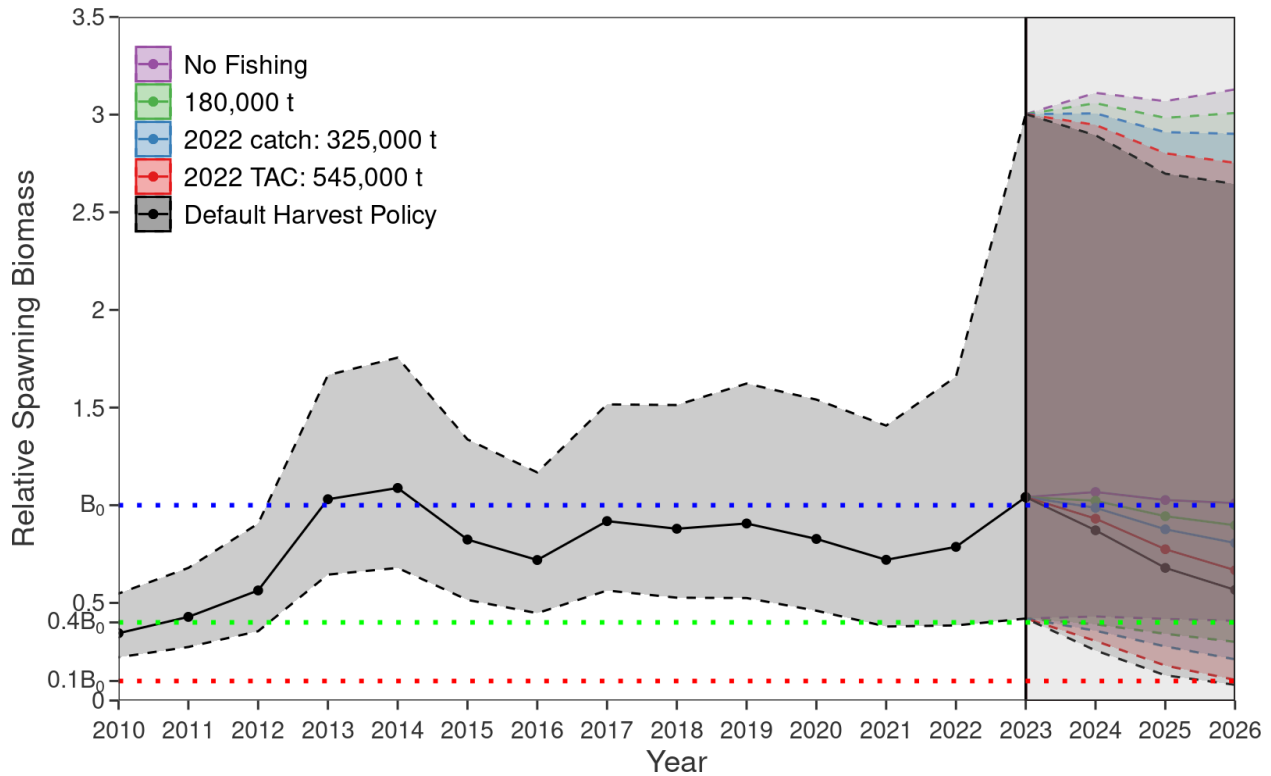
Figure j. Median and 95% posterior credibility intervals of estimated relative spawning biomass to the start of 2023 from the base model and projections to the start of 2026 for several management actions, which are defined in Table g.
