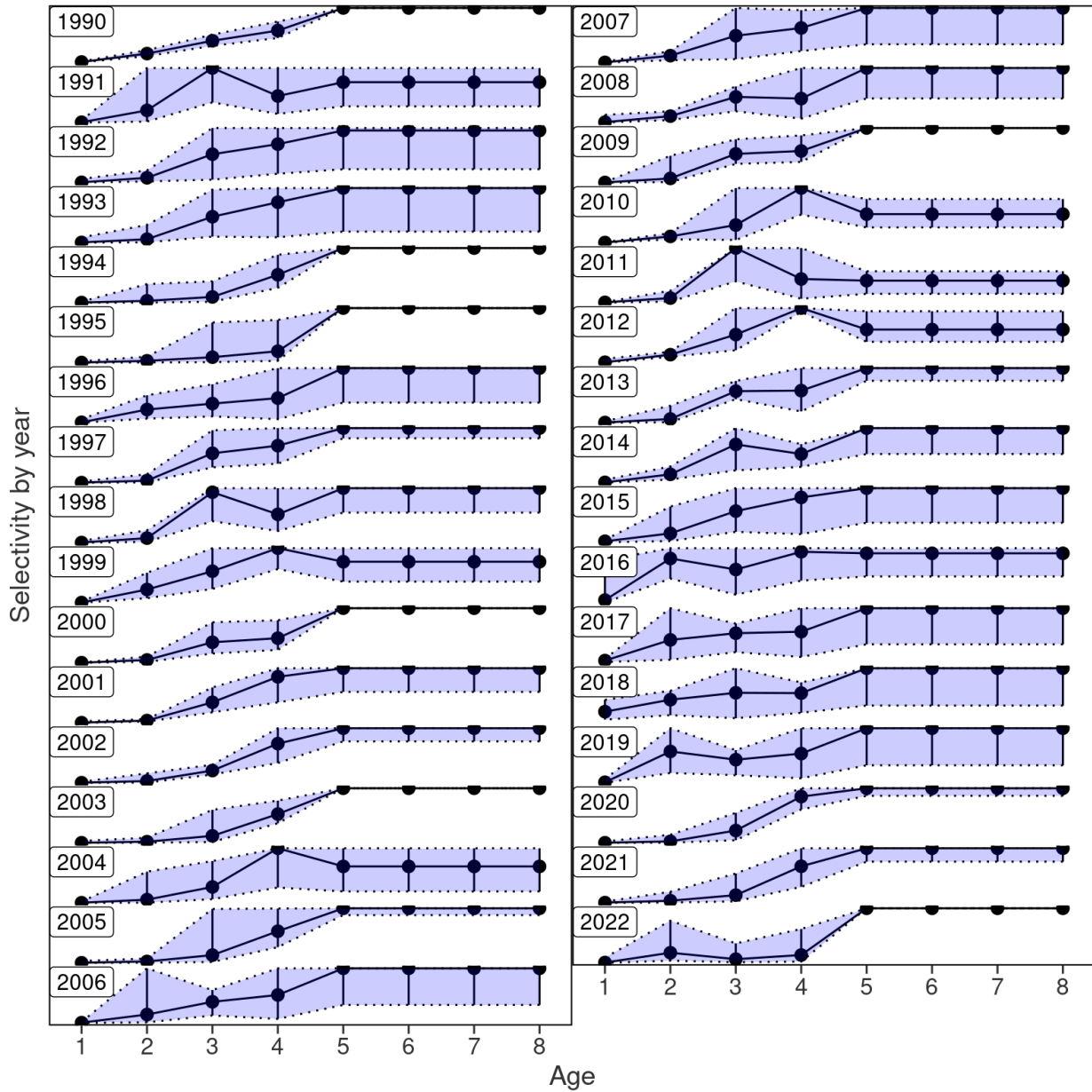
Figure B.4. Fishery selectivity sampled from posterior probability distribution by year for the sensitivity model with maximum age of estimated selectivity set to 5. Black dots and bars indicate the median and 95% credibility interval, respectively. The shaded polygon also shows the 95% credibility interval. Range is from 0 to 1 within each year. Selectivity for 1990 is shared for all years from 1966 to 1990.
