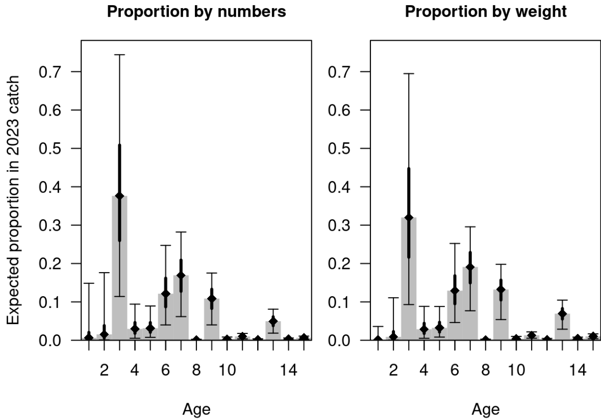
Figure 41. Forecast age compositions in numbers and in weight for the 2023 fishery catch (combined across all sectors in both countries). Gray bars show median estimates. Thick black lines show 50% credibility intervals and thin black lines show 95% credibility intervals. These estimates are based on the posterior distribution for selectivity averaged across the most recent five years, weight-at-age data averaged across the most recent five years, and the distribution for expected numbers at age at the start of 2023 (see Table 18 for the MCMC medians of numbers-at-age for all years). The panel on the right is scaled based on the weight at each age averaged across the last five years.
