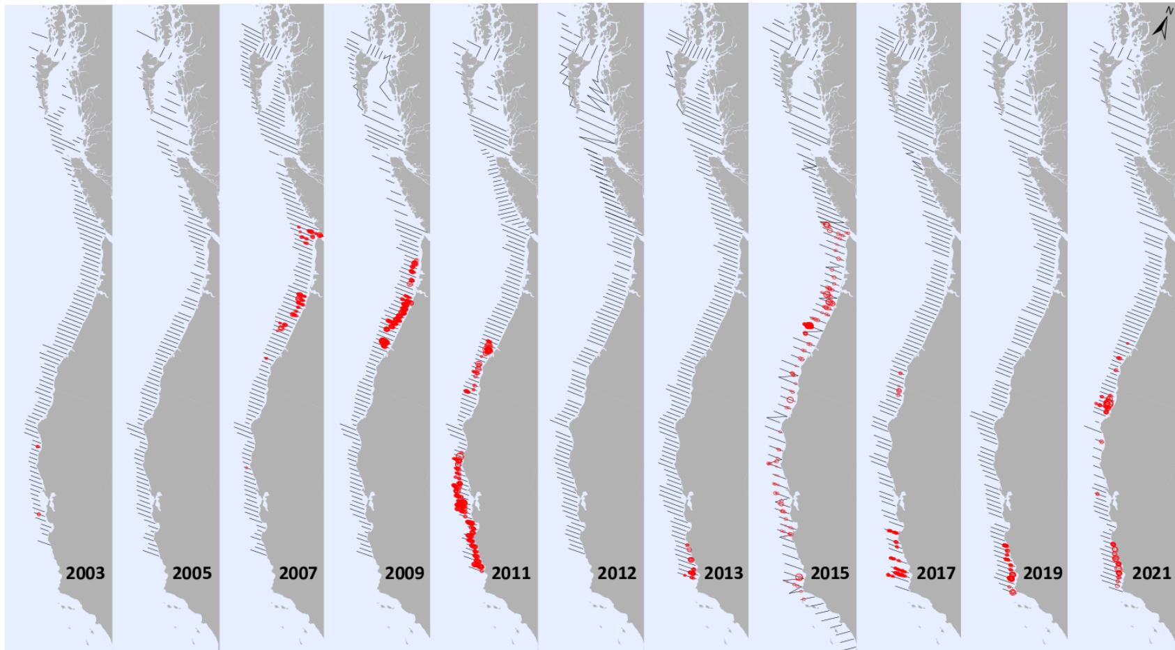
Figure 3. Spatial distribution of acoustic backscatter attributable to aggregations of age-1 Pacific Hake from the Joint U.S. and Canadian Integrated Acoustic and Trawl Survey 2003–2021 (spatial details are not available for survey years 1995, 1998, and 2001). Age-1 Pacific Hake are not fully sampled during the acoustic survey and were not explicitly considered during establishment of the survey sampling design. Additional backscatter from age-1 fish intermixed with older fish is not shown. Area of the circle is roughly proportional to observed backscatter. Figure produced by Julia Clemons (NOAA).
