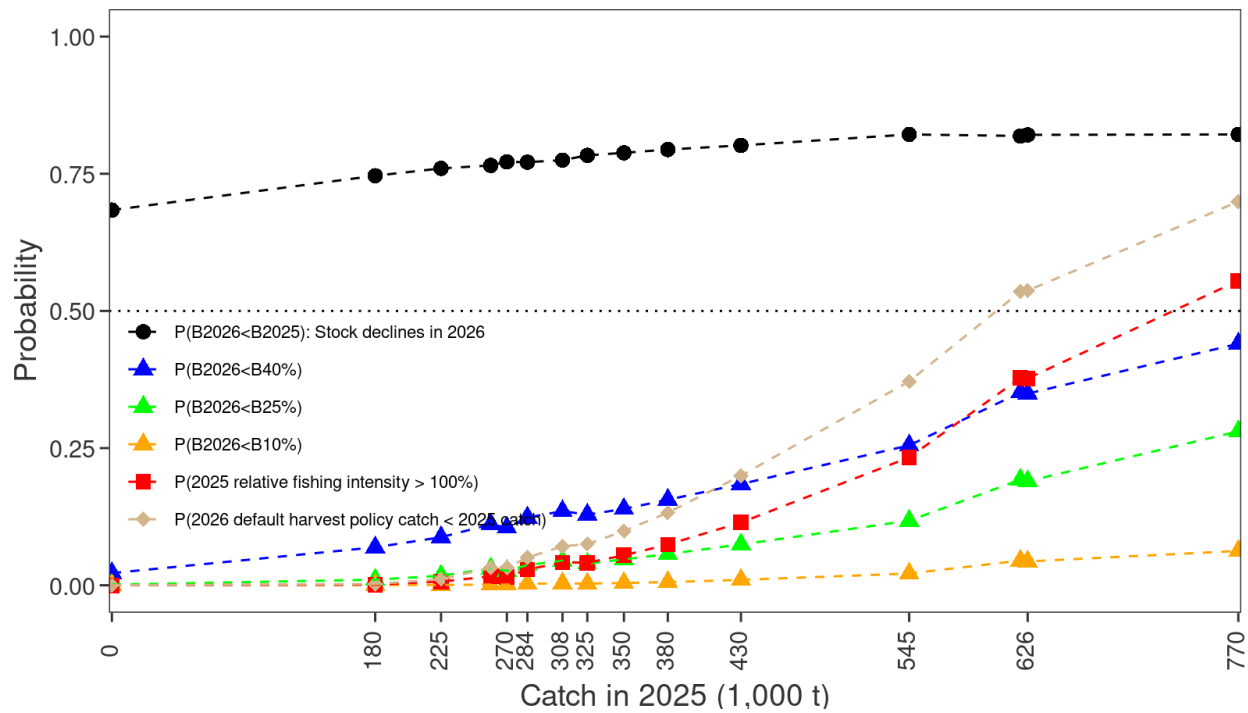
Figure 40. Graphical representation of the base model results presented in Table 32 for catch in 2025, given the 2023 and 2024 catch levels shown in Tables 30 and 31. The symbols indicate points that were computed directly from model output and lines interpolate between the points.
