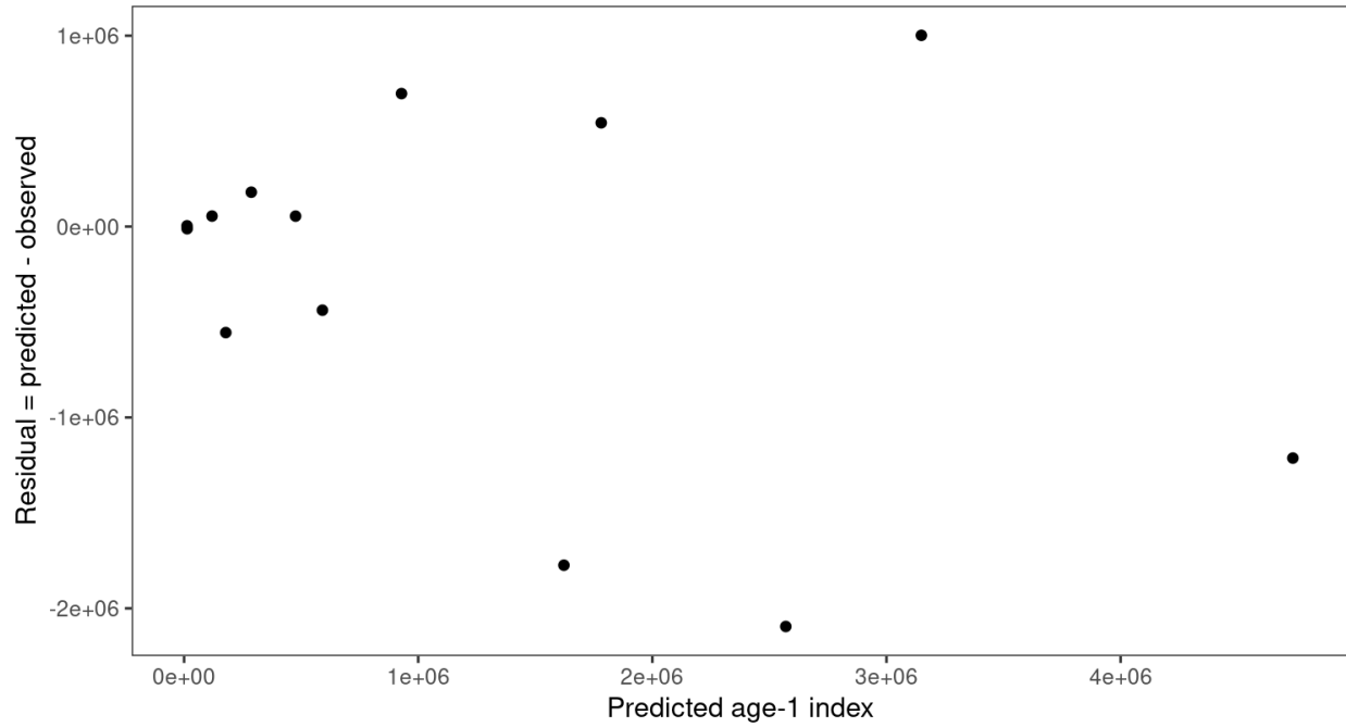
Figure B.1. Residuals of the age-1 index fits against the predicted values.
